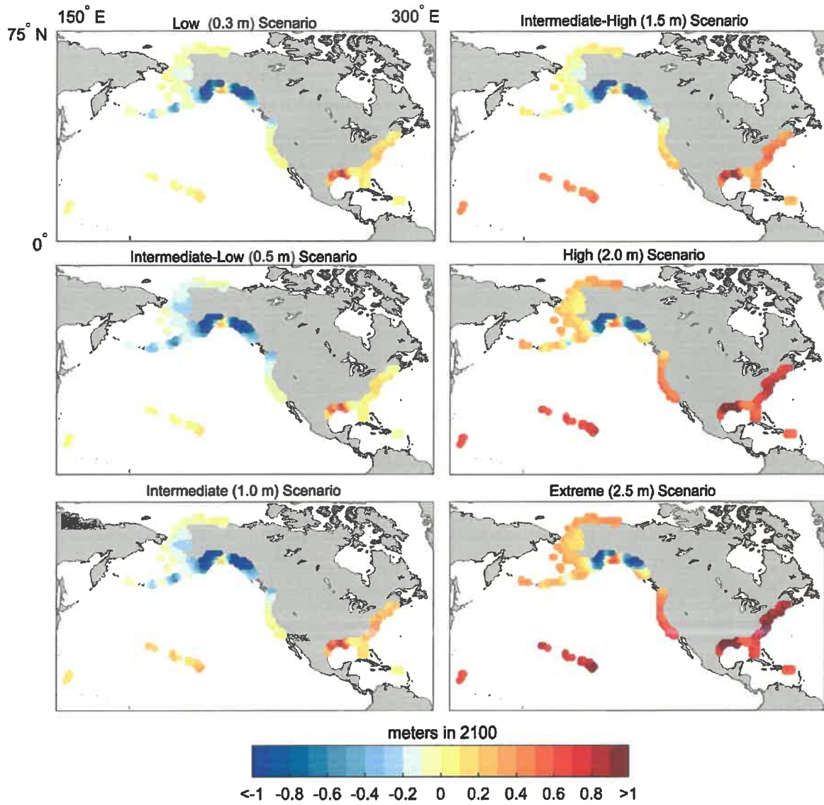
Figure 13. Total RSL change at 1-degree resolution for 2100 (in meters) relative to the corresponding (median-value) GMSL rise amount for that scenario. To determine the total RSL change, add the GMSL scenario amount to the value shown.
