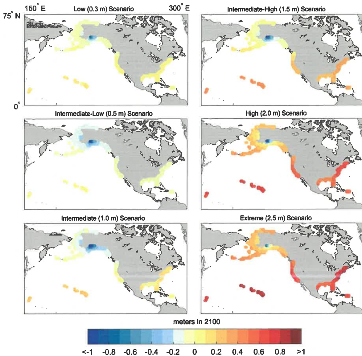
Figure 9. Climate-related RSL change at 1-degree resolution for 2100 (in meters) relative to the corresponding (median-value) GMSL rise amount for that scenario. To determine the total climate-related RSL change, add the GMSL scenario amount to the value shown.
