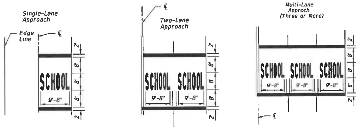
Figure 15-17B School Pavement Message Layouts for Single and Multi-Lane Approaches
