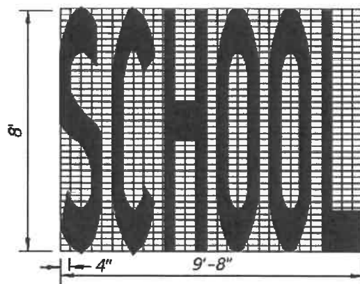
Figure 15-17A. School Pavement Message Details
