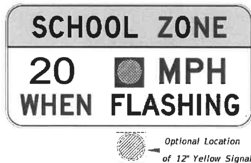
Figure 15-7D 20 MPH School Zone Flashing Beacon Assembly (Overhead Option FTP 31-06)
