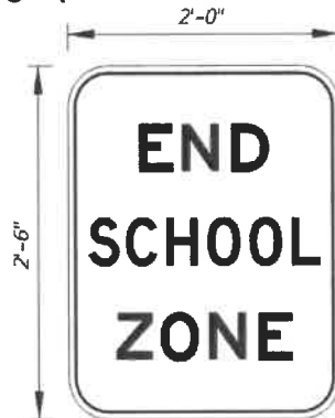
Figure 15-9A End School Zone Sign (Ground-Mounted Option – FTP 34-06)
