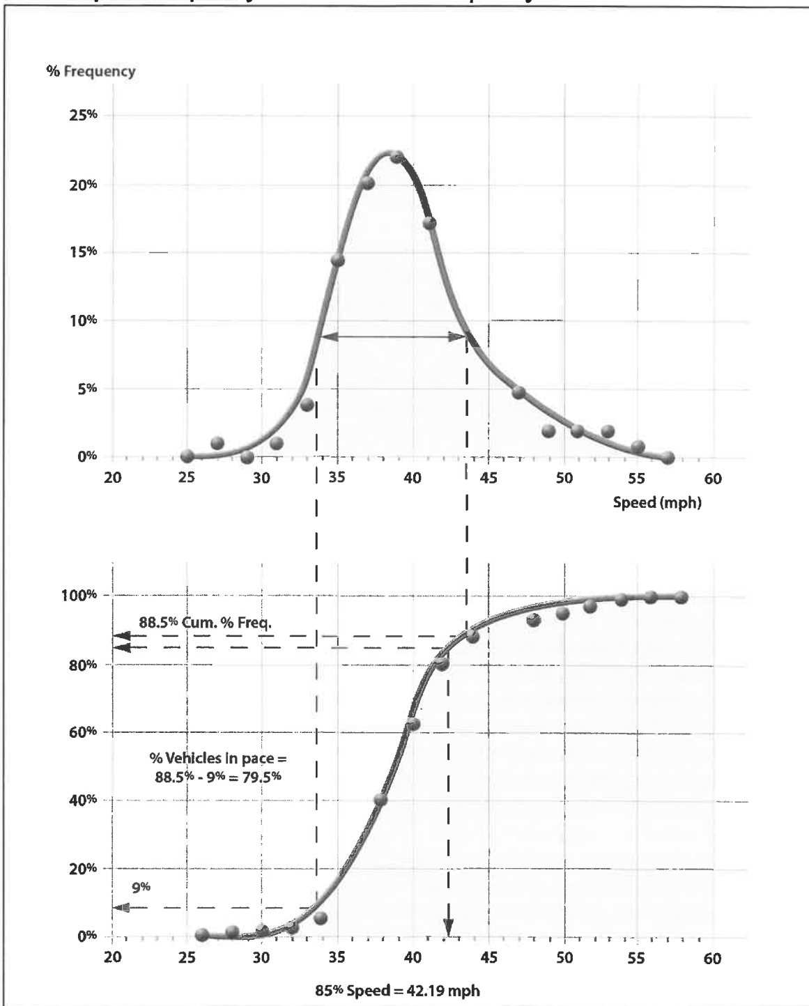
Figure 4-1 Speed Frequency and Cumulative Frequency Distribution Curves
