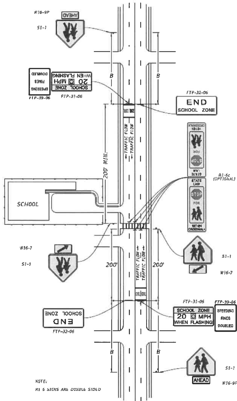
Figure 15-15 Typical School Zone With School Crossing (Multilane Undivided) (45 mph or less) Mid-block or on Thru Street at an Intersection
