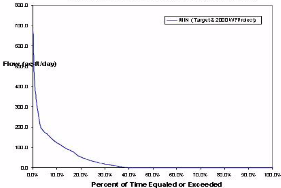
Figure &C. Simulated Surface Water Deliveries to Pumpkin Bay from Faka Union Flowway Near US 41 Dry Season Volume Probability Curve (Nov 1 - May 31)
