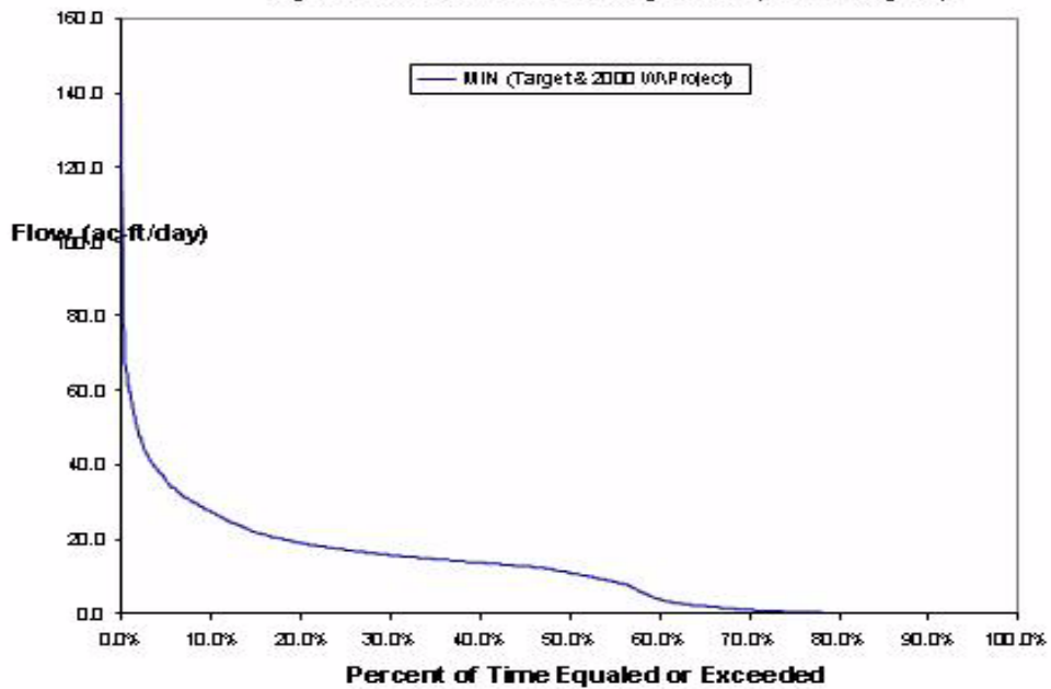
Figure 6.C. Simulated Surface Water Deliveries to Faka Union Bay from Faka Union FU#1 Near US 41 Dry Season Volume Probability Curve (Nov 1- May 31)
