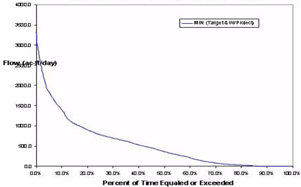
Figure 10. B. Simulated Surface Water Deliveries to Fakahatchee Bay from Fakahatchee Strand Wet Season Volume Probability Curve (June 1- Oct 31)
