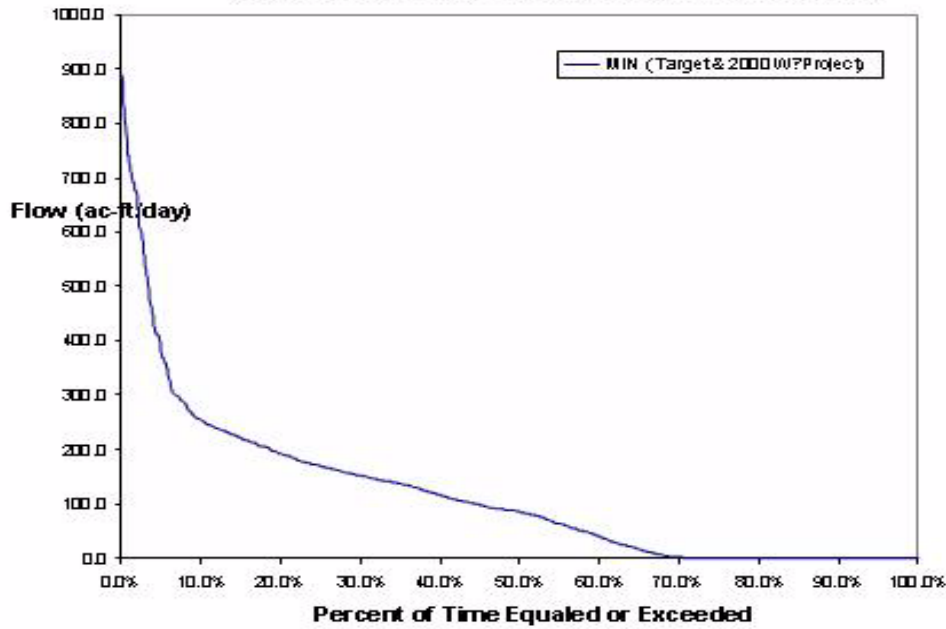
Figure &B. Simulated Surface Water Deliveries to Pumpkin Bay from Faka Union Flowway Near US 41 Wet Season Volume Probability Curve (June 1 - Oct 31)
